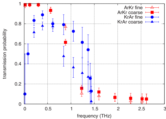
FIG. 8. (Color online) Transmission coefficients of wave-packets propagating from argon and krypton into the opposite as a function of frequency in diffuse interfaces.
