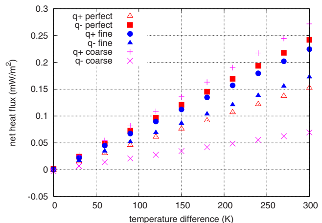
FIG. 10. (Color online) Net flux in the positive and negative directions calculated based on Eq. (9) with the transmission coefficients calculated from molecular dynamics simulations.
