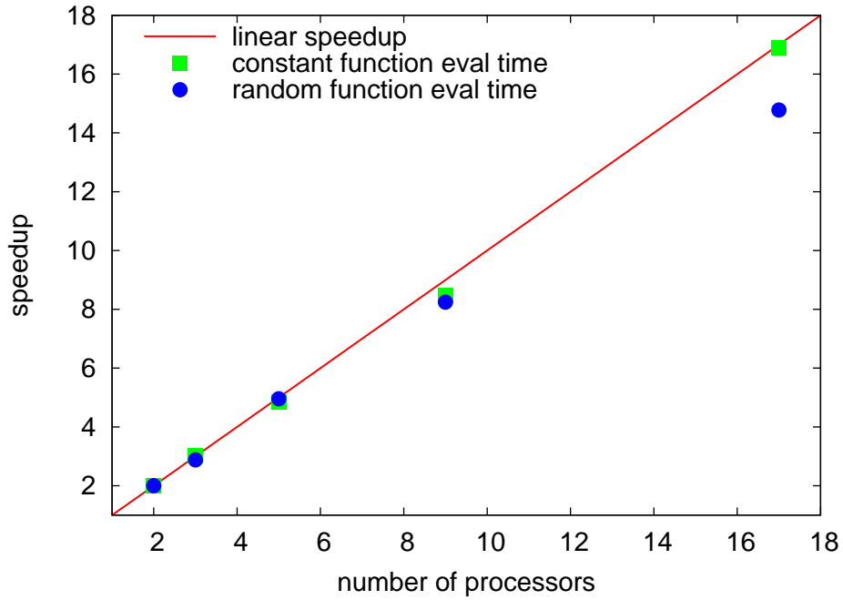
Figure 1: Speedup measured for a constant function evaluation time and a random function evaluation time (from 0 to 5 seconds of sleep).
