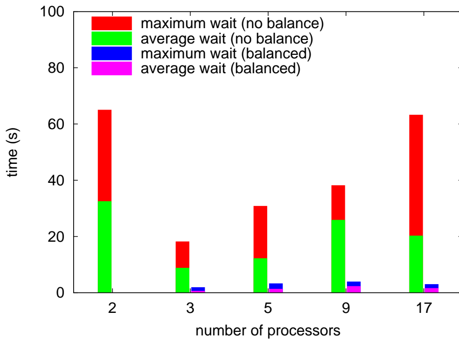
Figure 2: The maximum and average wait times for a non-balanced case and when load balancing is employed.
